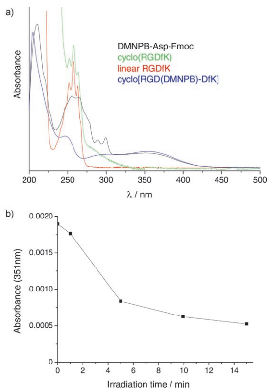
Figure 1. a) UV spectra of DMNPB-Asp-Fmoc, cyclo(RGDfK), linear RGDfK, and cyclo[RGD(DMNPB)fK] in solution. b) UV absorption measured at 351 nm for substrates modified with cyclo[RGD-(DMNPB)fK] after irradiation at 351 nm for different periods of time and washing. The decay in the absorption values corresponds to the cleavage of the chromophore from the surface during exposure to light.
