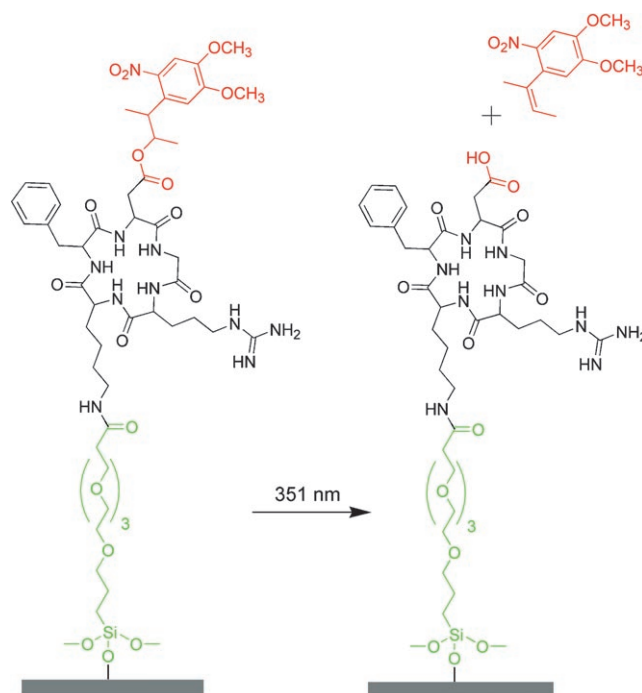
Scheme 1. Chemical structure of cyclo[RGD(DMNPB)fK] (DMNPB in red) attached to the surface through the TEG linker (green). The caging group is released upon irradiation at 351 nm.
